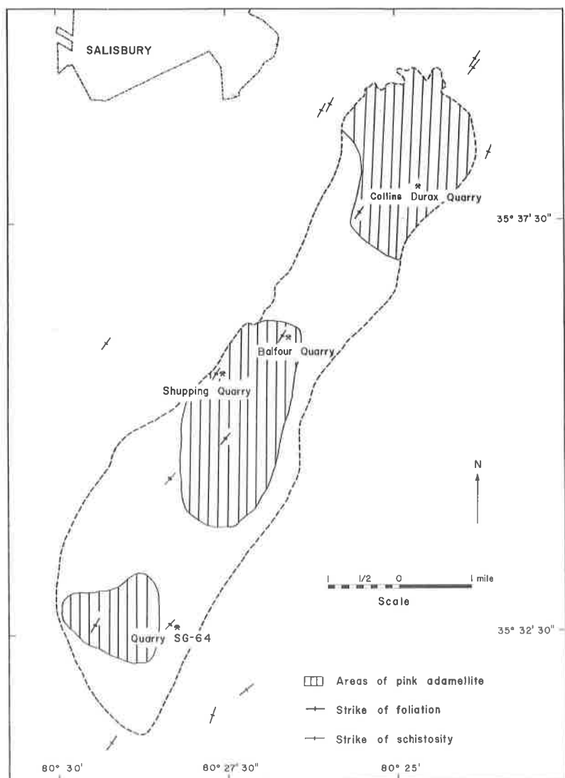
Figure 2. Geologic map.
