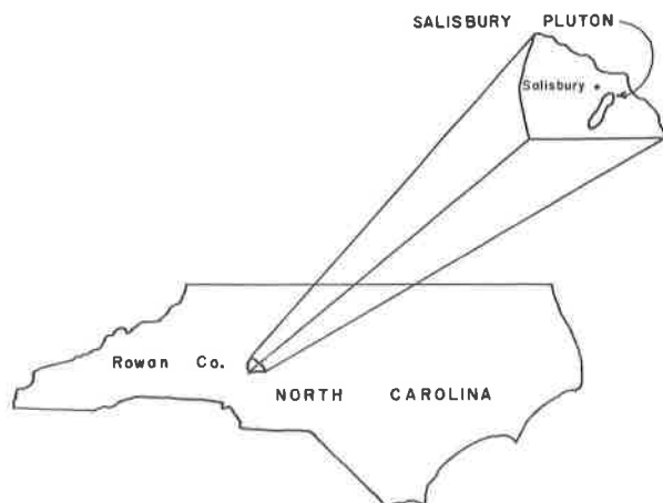
Figure 1. Index map.
