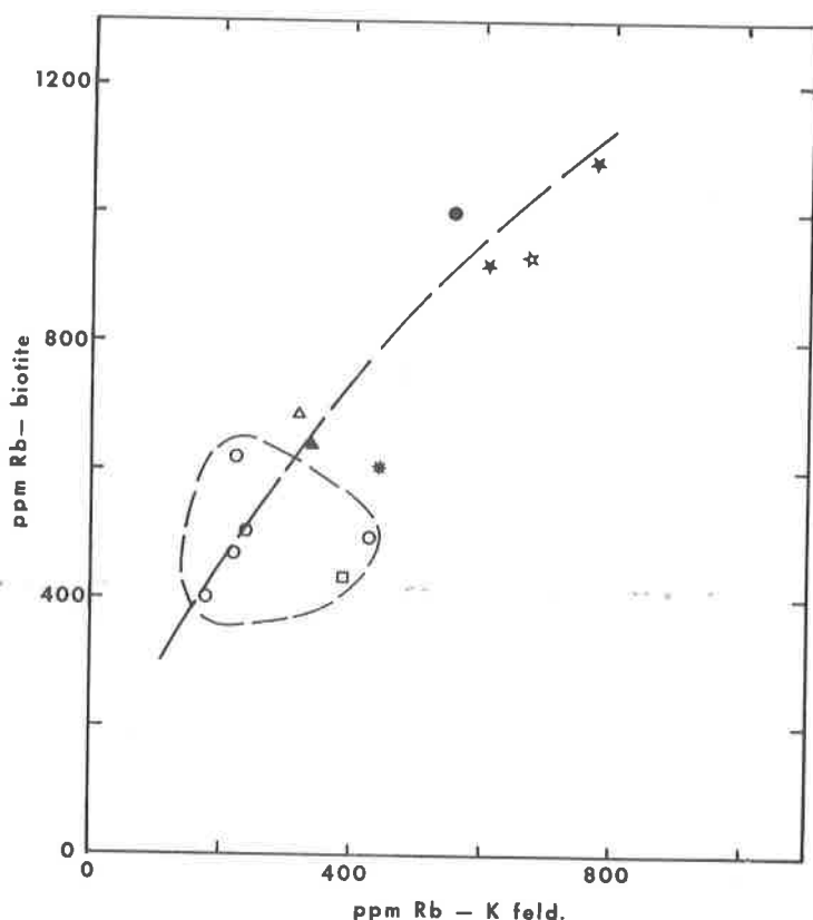
Figure 14. Plot of Rb in coexisting biotites and K-feldspars.
