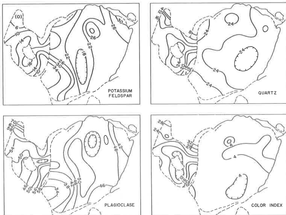
Figure 4. Contour maps of mineralogical variations, based on the raw data. Volume percent. Contour interval 4 percent.
