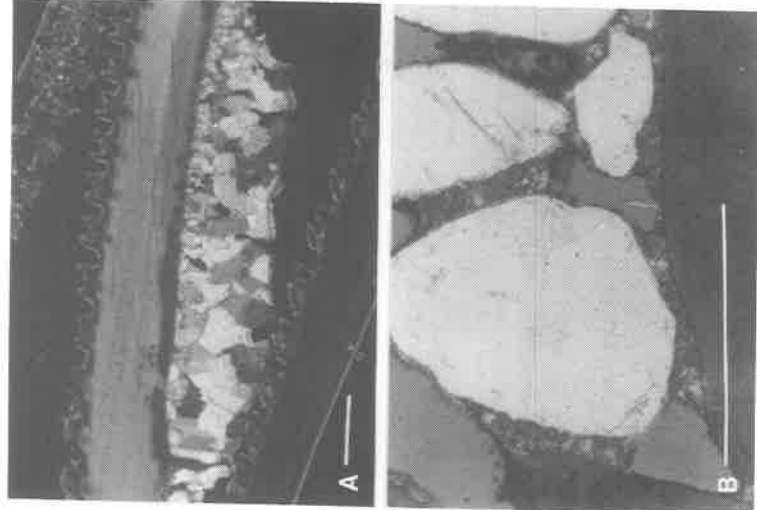
Figure 5. Photomicrographs of microborings in bioclasts taken from the unlithified shell hash at Snows Cut. (A) Nassarius obsoleta and (B) unidentified rounded shell fragment. Bars = 0.5 mm.
