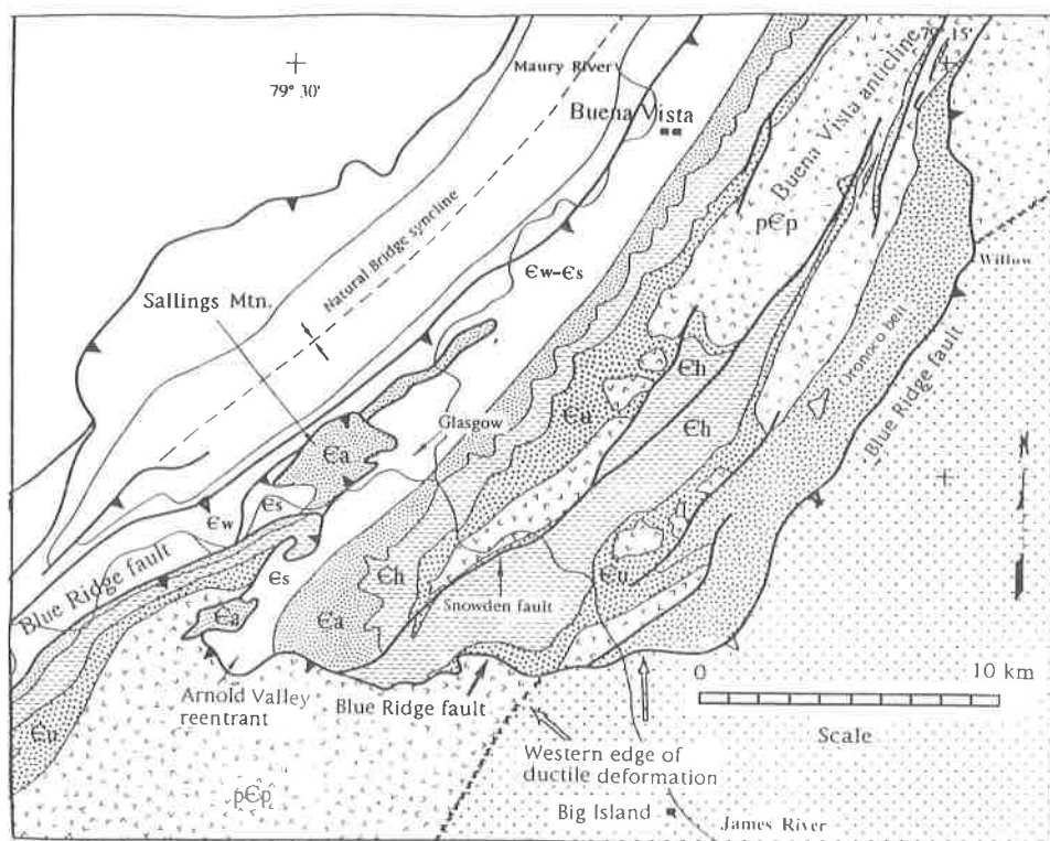
Figure 2. Tectonic sketch map of the northwestern flank of the Blue Ridge in the vicinity of the James River. Precambrian basement rocks are subdivided into two parts -- the Pedlar massif (v pattern) is largely composed of charnockitic rocks and granulite gneiss and the Lovingson massif (+ pattern) includes late Precambrian granites, diorites, quartzo-feldspathic veins, and quartz veins as well as charnockitic rocks and granulite gneiss. A number of zones of ductile deformation are present in the Lovingson massif. Thrust faults are indicated by heavy lines. Units of the Chilhowee (Antietam, Harpers, and Weverton (also Unicoi) Formations are distinguished by patterns. The Oronoco belt contains the Catoclin Formation and sedimentary rocks that resemble the Harpers and Weverton Formations. The younger sedimentary cover rocks in the Valley and Ridge are unadorned and largely undifferentiated. (Compiled from geologic maps by Spencer, 1968 and in press, and unpublished mapping by the author).
