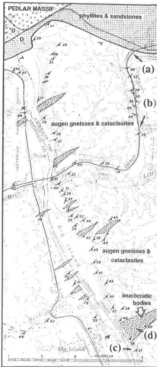
Figure 7. Sketch map of the ductile deformation zones exposed along the James River near Big Island, Virginia. Examples of representative rocks in the zone of ductile deformation are indicated. (a), folded mylonite from a locality near the Blue Ridge Parkway where the Blue Ridge thrust cuts the zone of ductile deformation. (see Figure 10C); (b), augen gneiss with drawn out porphyroclasts (see Figure 8B); (c), slightly deformed coarse-grained granitic rock in one of the lens-shaped bodies in the ductile deformation zone. (see Figure 8D); (d), small boudin composed of granitic rock enclosed in mylonite. (See Figures 12A and 12B).
