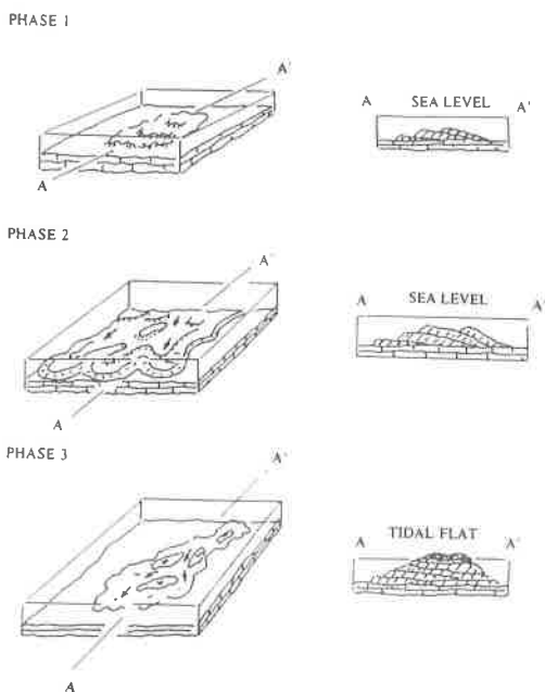
Figure 12. Three phase development of tidal bars in outcrops of Monteagle Limestone, after Handford (1978).
