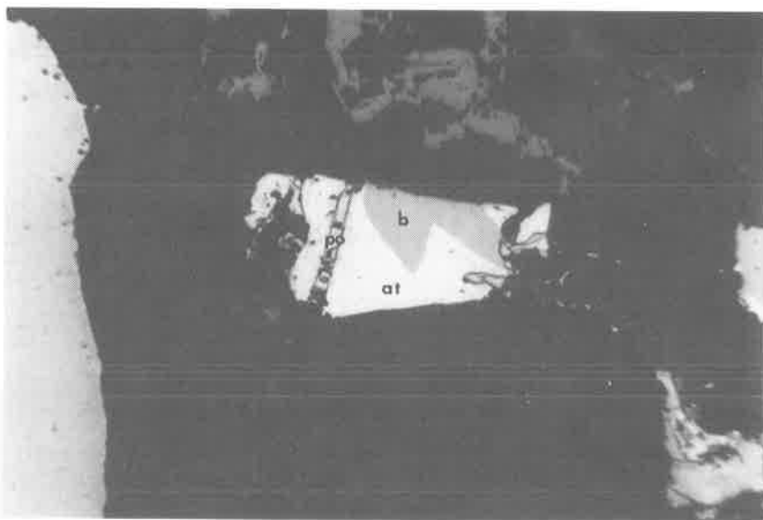
Figure 4. Photomicrograph of altaite ( \text{PbTe} ) (at) with boulangerite ( \text{Pb}_5\text{Sb}_4\text{S}_{11} ) (b) cut by a small veinlet of pyrrhotite (po). Kings Mountain, N.C.; field of view = 0.60 mm.
