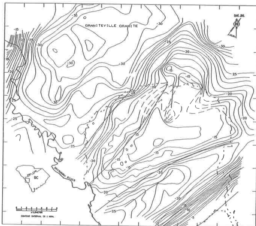
Figure 4. Gravity map of central Savannah River area.
