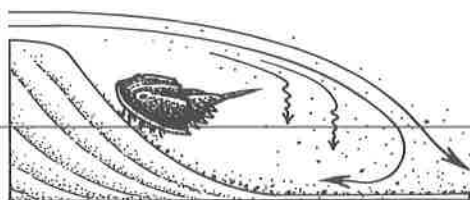
Figure 7. Lee-side velocity shadows might have provided shelter for feeding arthropods during periods of low current energy when the dunes had ceased to migrate. Nutrients might also have fallen out of separation eddies at the crest of the dunes or accumulated at the toes of the foreset following grain avalanching.
