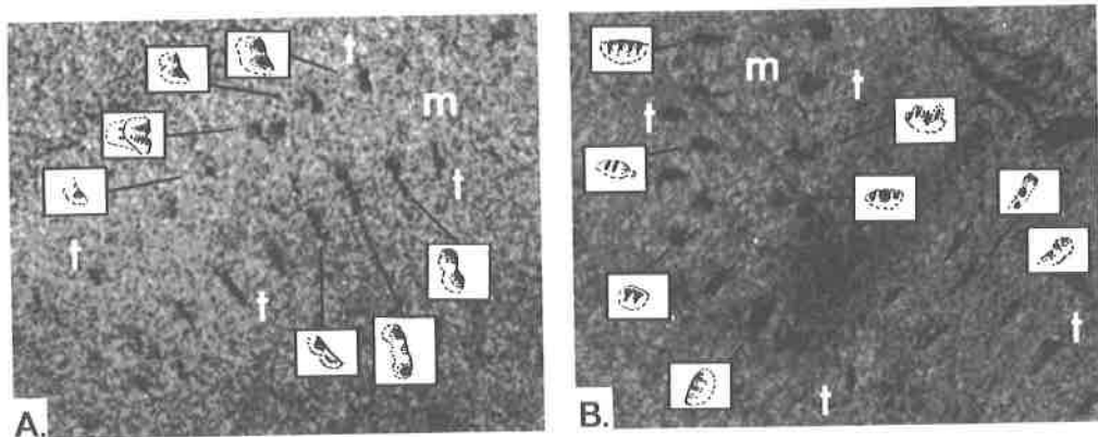
Figure 4. Photographs of trackways at location B. Inset illustrations show details (black indicates deeper indentation). The trackways (A-B) are composed of pairs of transverse indentations (T) that may contain three to four smaller marks (see insets) separated by featureless medial axes (M). One of the tracks (B) shows evidence for a side-step (arrow) during ascent.
