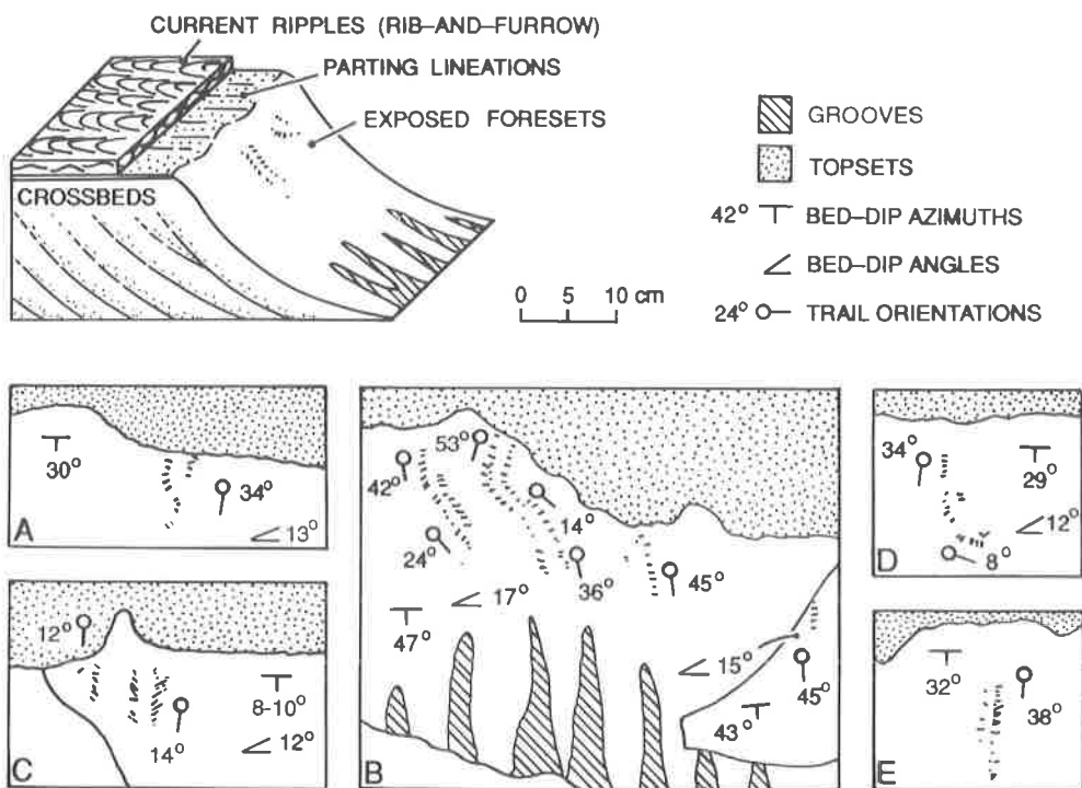
Figure 5. Sketches of tracks A, B, C, D, and E in Figure 3. All tracks occur on inclined foresets. Each figure is oriented parallel to bed dip.
