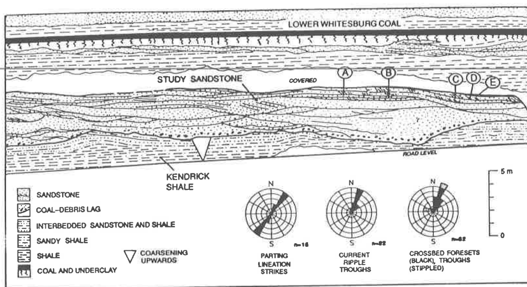
Figure 3. Illustration of the track-bearing sandstone based on an outcrop photomosaic showing the position of walking traces (A, B, C, D, and E) in Figure 4, and rose diagrams of various sedimentary structures in the track-bearing sandstone.
