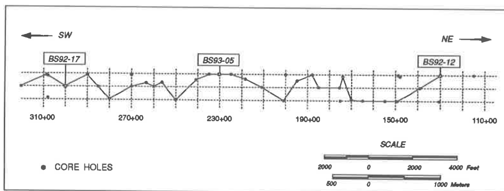
Figure 2. Core-hole locations along Bald Head Shoals Channel, Long Bay, with three cores identified for reference. Line connecting core holes represents the line of section that is shown in Figure 3. The three parallel dashed lines approximate the channel margins and the channel center. Locational data is the U. S. Army Corps of Engineers scheme and is given in feet. For example, the distance between 150+00 and 190+00 is 4000 ft. Location of core-holes in latitude and longitude is given in Appendix A.
