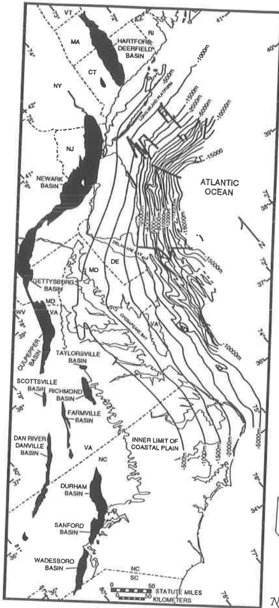
Figure 1: Map of the Exposed Newark Supergroup Basins in the Eastern United States, the basins are shown by solid black. State abbreviations are: CT= Connecticut, DE= Delaware, MA= Massachusetts, MD= Maryland, NC= North Carolina, NJ= New Jersey, NY= New York, PA= Pennsylvania, RI= Rhode Island, SC= South Carolina, VA= Virginia, VT= Vermont, WV= West Virginia; and C. H.= Cape Hatteras. Contours indicate depth of sedimentary section, (after Benson, 1984).
