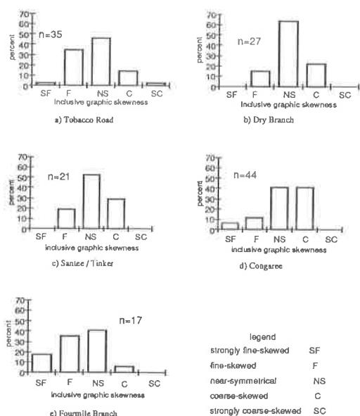
Figure 8.-Distribution of inclusive graphic skewness (Folk and Ward, 1957) for stratigraphic units at the MWD Well Field as determined by sieve analysis.
