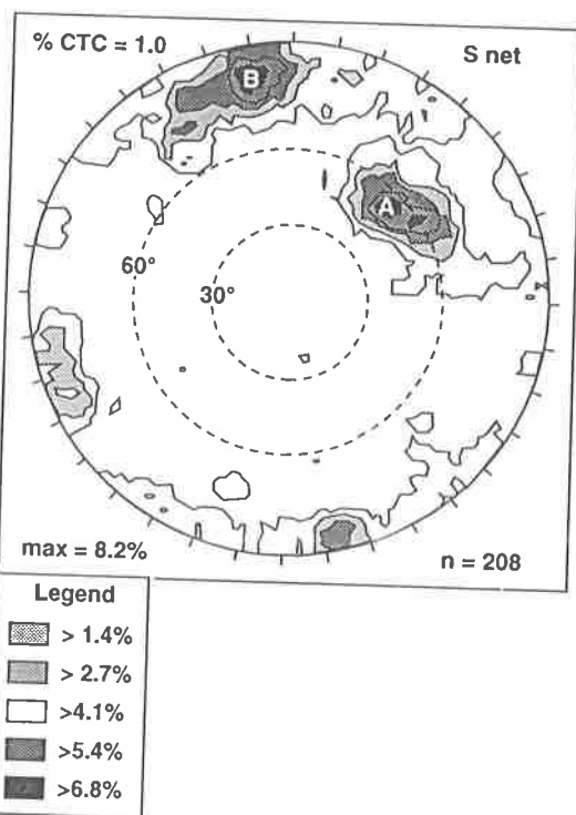
Figure 6: Contour plot of 208 joint poles plotted as percent per one percent of total area. The plot reveals two joint sets at N40^{\circ}W , 50^{\circ}SW , and at N70^{\circ}E , 80^{\circ}SE .
