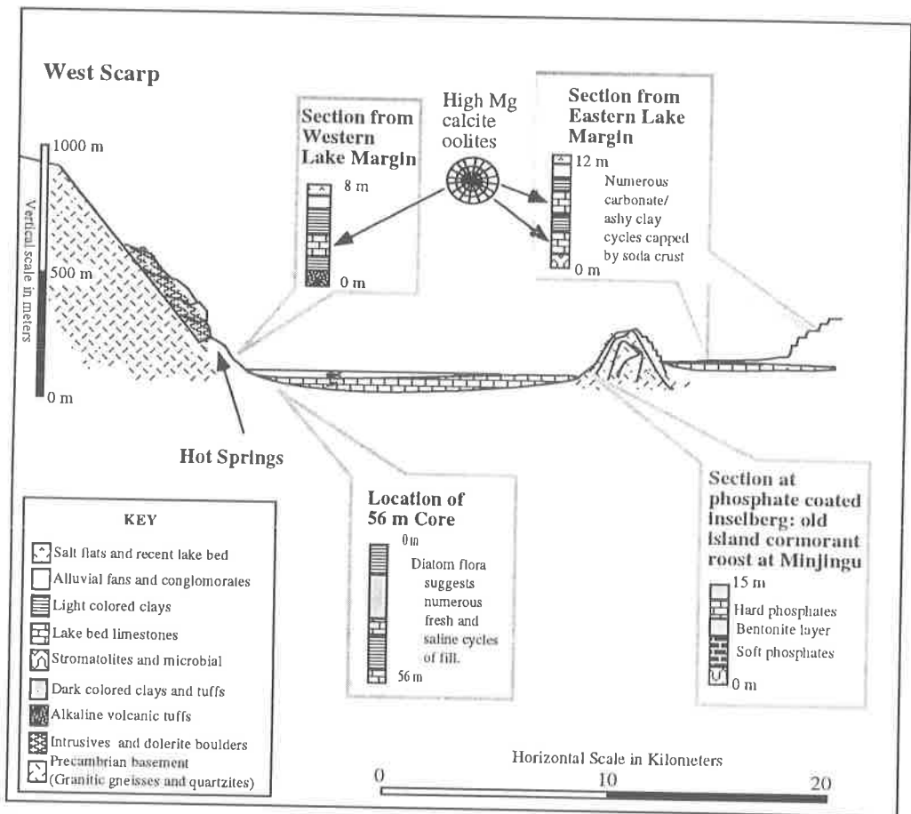
Figure 2. Schematic cross section of Lake Manyara showing the major sedimentary character of valley fill.
