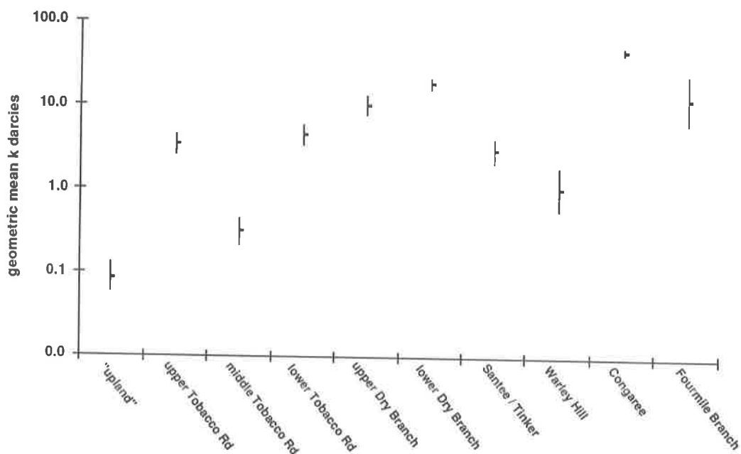
Figure 19.-Geometric mean permeability for units in the MWD Well Field. Error bars represent 95% confidence interval.
