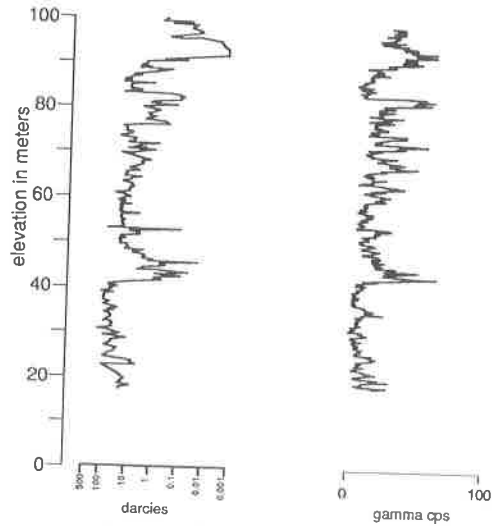
Figure 12.-Permeability profile and gamma ray log for well MWD 2.
