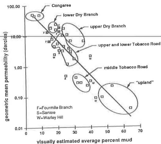
Figure 11.-Plot of visually estimated mud content versus geometric mean permeability.
