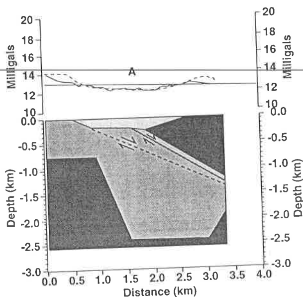
Figure 19: Gravity model developed for the U.S. Highway 60 gravity profile. The lower section gives the geological model. The upper section gives the observed and the calculated anomalies. A: Triassic basin.
