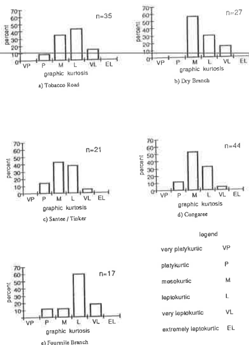
Figure 9.-Distribution of graphic kurtosis (Folk and Ward, 1957) for stratigraphic units at the MWD Well Field as determined by sieve analysis.
