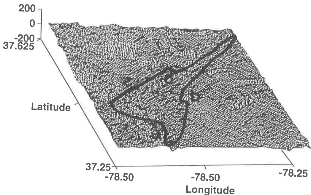
Figure 14: A three dimensional view of the second derivative of Bouguer gravity field over the Farmville Basin. Letters a-d indicate various structures; a: dike; b: probable dike; c: mylonite; and d: probable mylonite.
