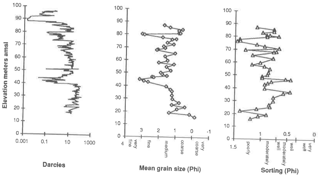
Figure 15.-Permeability profile for well MWD 2 with mean grain size and sorting profiles.
