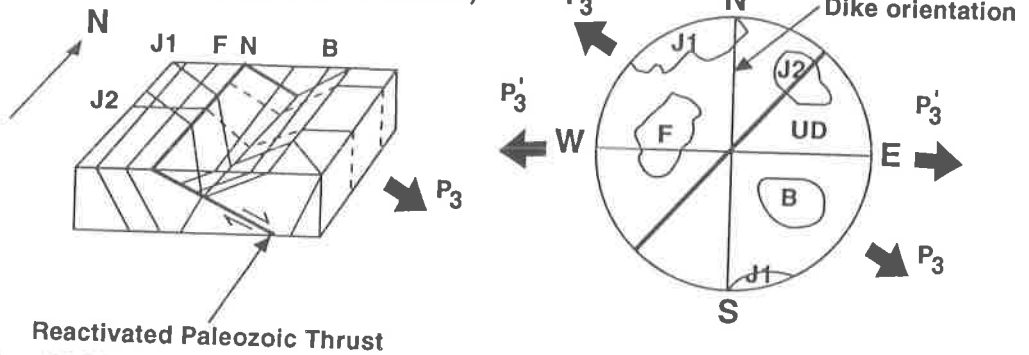
Figure 23: Kinematic model for evolution of the Farmville Basin. The simplified block diagram illustrates the major structural features together with the associated stereonet projections. P1: compressional axis; P3: tensional axis, P'3: tensional axis after rotation; T: thrust fault, N: reactivated thrust fault; F: foliation; J1: NE-SW release fractures; J2: E-W extension joints; B: bedding.
