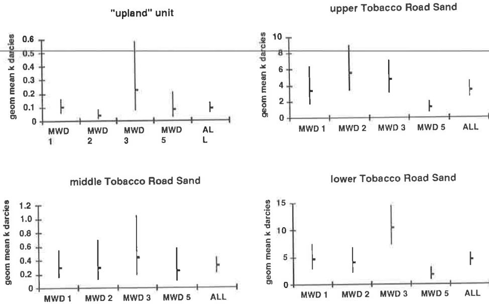
Figure 20.-Geometric mean permeability of the upper units in the MWD Well Field. Error bars represent 95% confidence interval.
