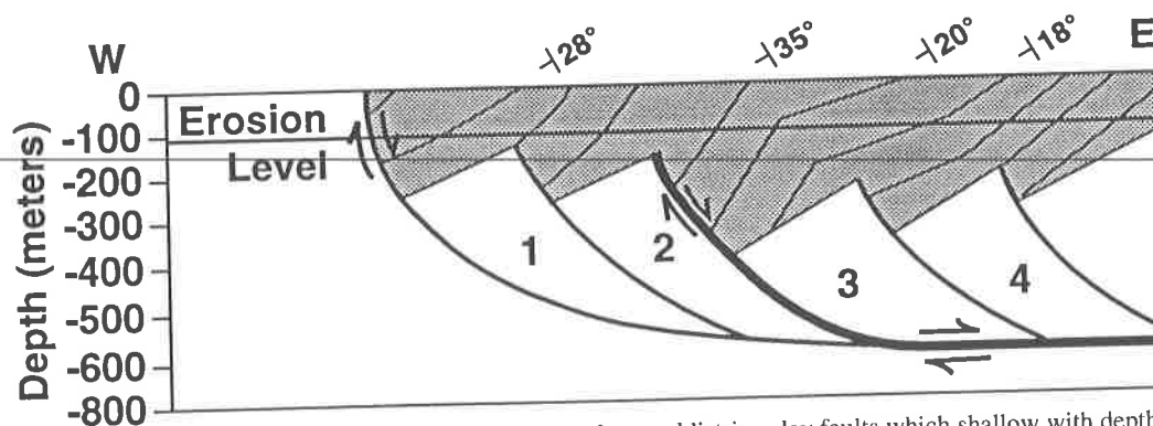
Figure 22: The Farmville Basin is formed as a result of several listric splay faults which shallow with depth and eventually join the master fault at depth. Light solid lines: dip of Triassic beds; dotted area: Triassic rocks; heavy line: master fault; Intermediate solid line: splay faults; 1,2,3, and 4: fault blocks. Approximate positions of observed dip on the surface are indicated. This model is similar to the model developed for State Road 636 gravity profile. Vertical exaggeration is about 32.5 percent.
