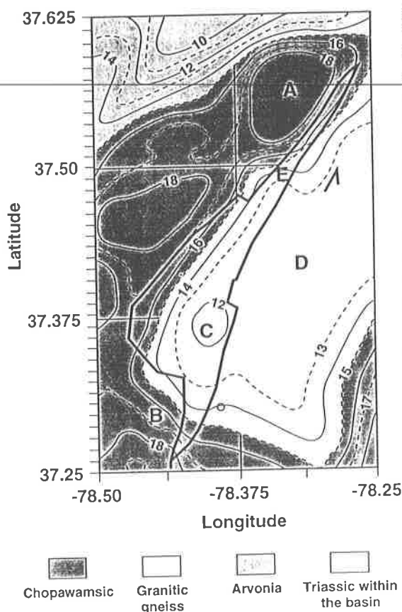
Figure 13: Interpretation of the subsurface basement of the study area using the upward continuation of the gravity field. We have chosen the 15 mgals contour line as an approximate border line between various lithologies, because this was observed at the 8 km level. This map is very close to the map of Marr (1980) and Brown (1969).
