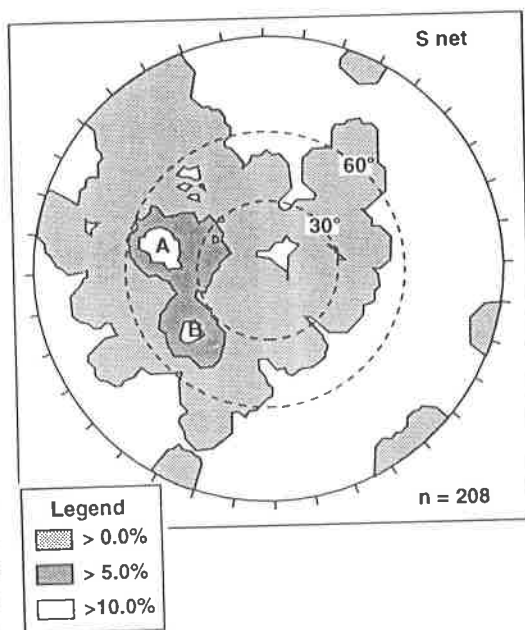
Figure 4: Contour plot of 208 poles to foliation from this study and the geologic map of Marr (1980). Contour plot of poles to foliation plotted as percent of per one percent of total area. The maxima represent foliation planes located at N15°E, 35° SE, and N40°W, 35° NE. Pole maxima are separated by 35 degrees azimuth. The distribution of pole clusters shows that the approximate average foliation plane strikes nearly north-north-east and dips to the south east.
