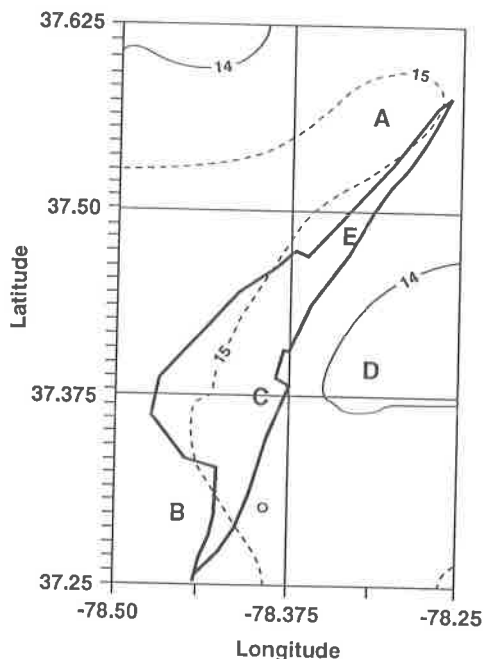
Figure 12: Upward continuation of the Bouguer gravity anomaly field at level of 8 km. At this level barely the NE-SW trend associated with the western border fault is observed, thus this is the most pronounced feature of the basin.
