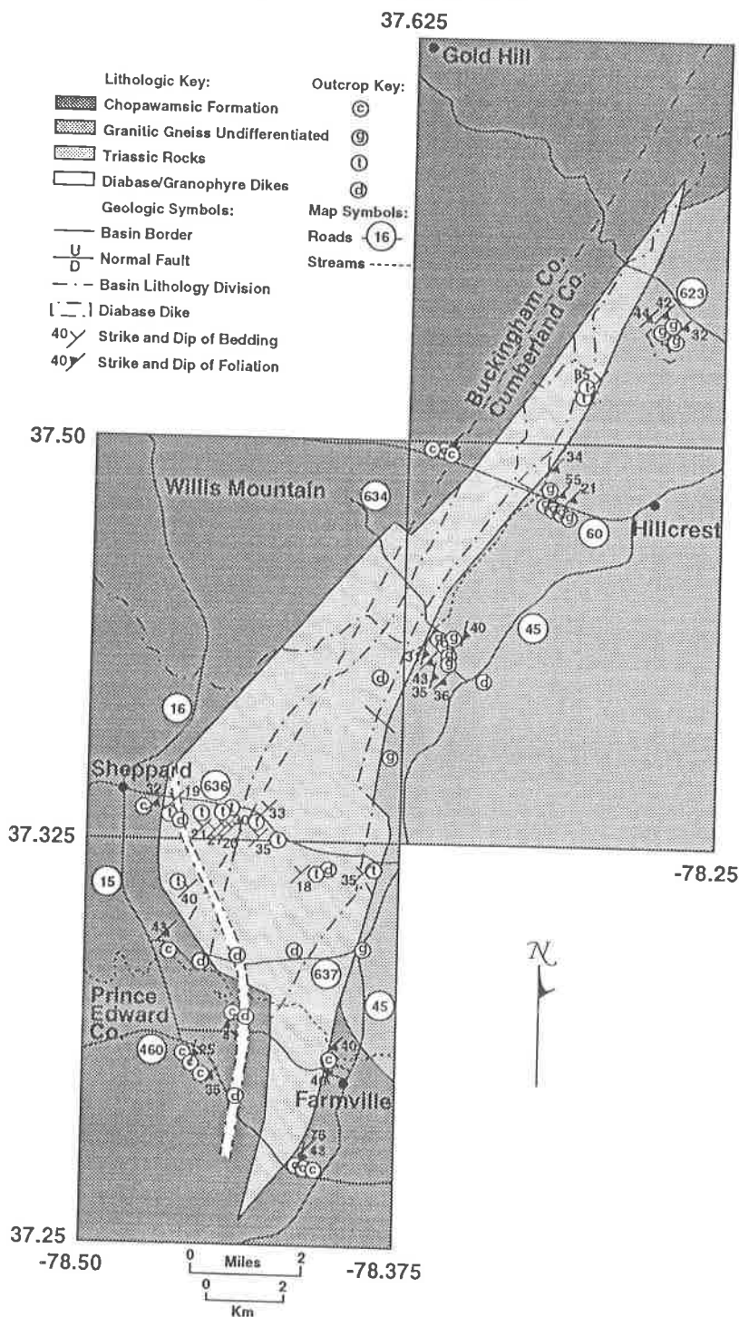
Figure 3: Geology map of the Farmville Basin. This map is based on the work of Marr (1980, 1981), and Brown (1969) as well as field investigation conducted for this study.
