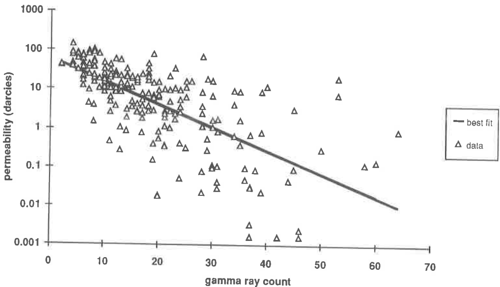
Figure 13.-Plot of permeability versus gamma ray count for well MWD 2.
