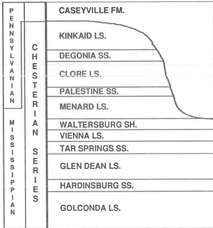
Figure 3. Stratigraphic column of the study area.
