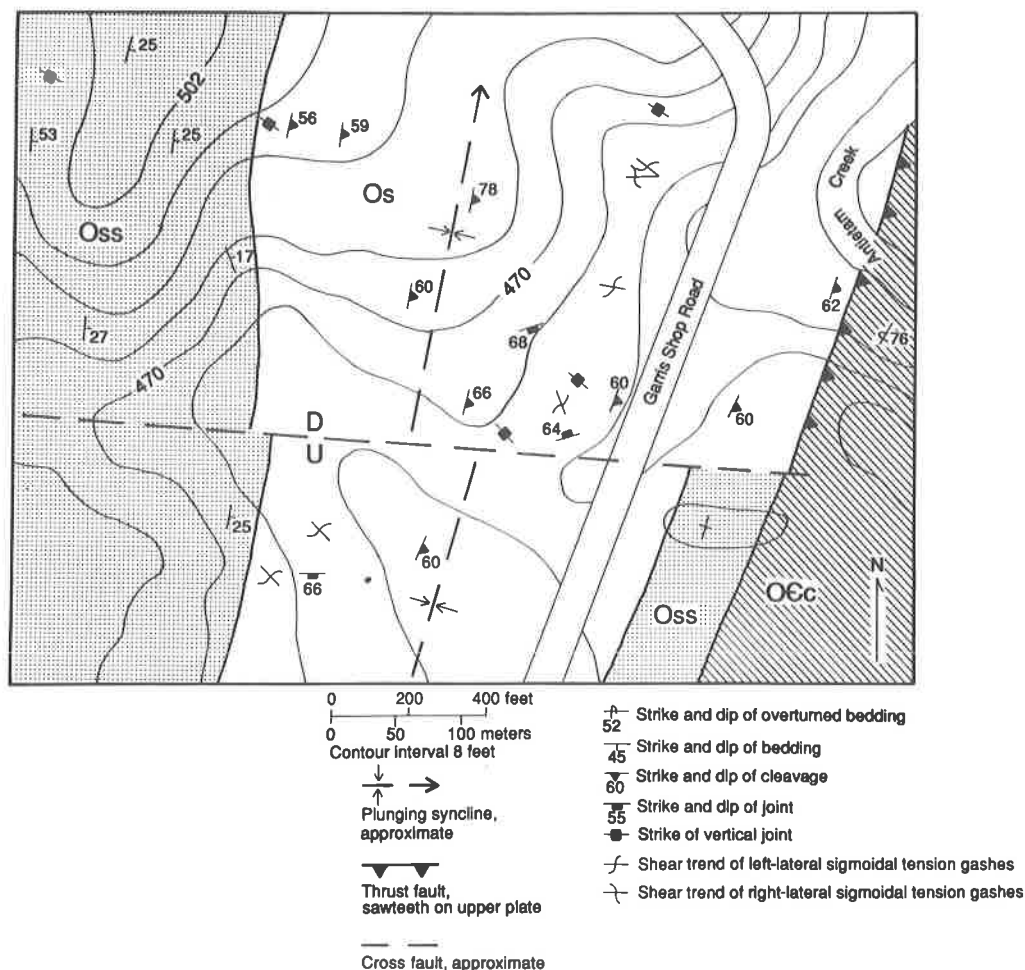
Figure 5. Detailed geologic map of the Funkstown cross fault, Washington County, Maryland (B on figure 1). OCco, Conococheague Limestone (Upper Cambrian and Lower Ordovician); Os, Stonehenge Limestone (Lower Ordovician); Oss, Stoufferstown Member of Stonehenge Limestone.
