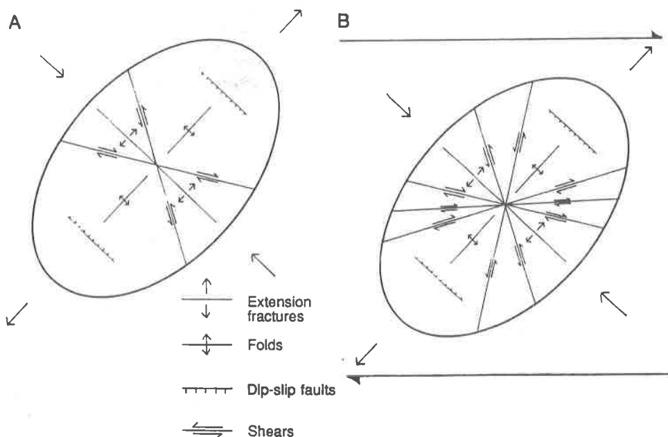
Figure 11. Strain ellipse diagram of, A, structures characteristic of pure shear, and, B, structures characteristic of simple shear (modified from Hancock, 1985, and Sylvester, 1988).
