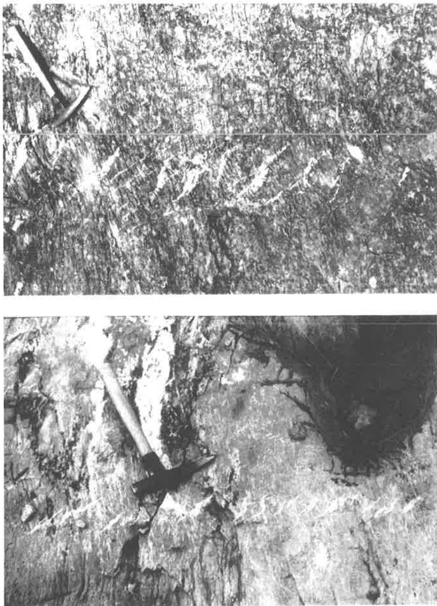
Figure 4. Photographs of set 1 sigmoidal tension gashes on horizontal pavement outcrops in the Rocky Marsh cross fault zone. Direction of shearing is left lateral on both sets. Handle of rock hammer points north.
