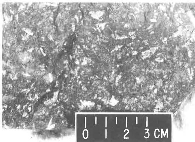
Figure 4. (A) Columnar jointing, common in many of the basaltic flows. (B) Amygdaloidal portion of a flow. (C) Porphyritic basalt, collected from near Cedar Run Trail, east of Hawksbill Mt. traverse.
