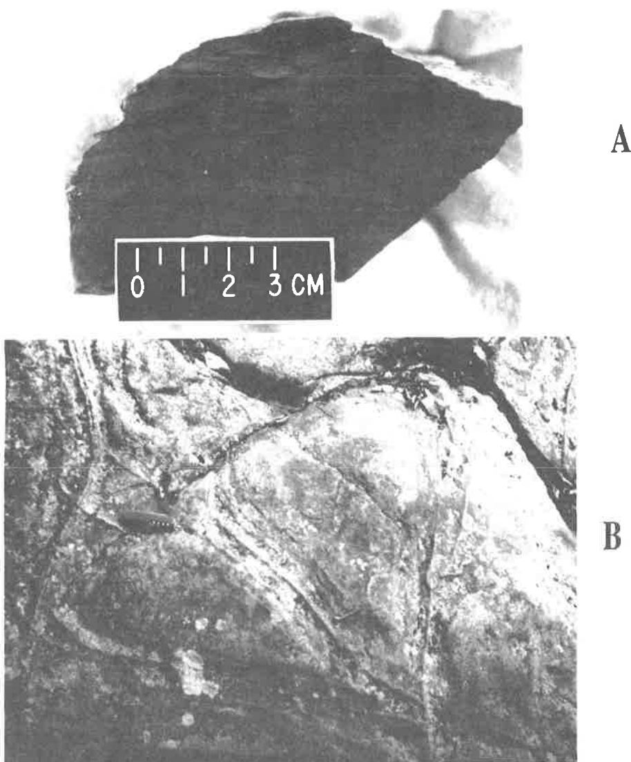
Figure 6. (A) Purple phyllite, locally found as thin interbeds between flows, and interpreted as felsic ash-flow tuffs or ignimbrites. (B) Pillow lava, located at Dark Hollow Falls, east of Big Meadows traverse.
