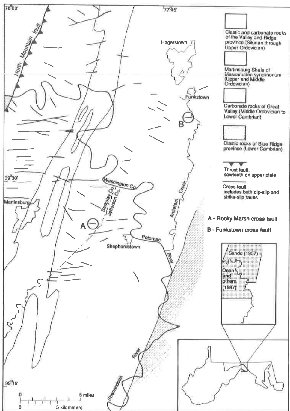
Figure 1. Generalized geologic map of the Great Valley of Maryland and West Virginia showing mapped cross-strike faults of Sando (1957) and Dean and others (1987) and locations of Rocky Marsh cross fault (A) and Funkstown cross fault (B).
