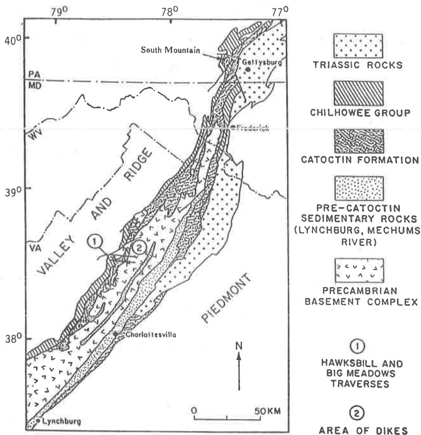
Figure 1. Index map of the central Appalachian Mountains showing location of the Catoctin volcanic province, along with geographic locations of the Blue Ridge Province, Valley and Ridge, and Piedmont. Location of study area near Luray, Va. is shown, along with the general location of many of the mafic dikes. Adapted from Reed and Morgan (1971).
