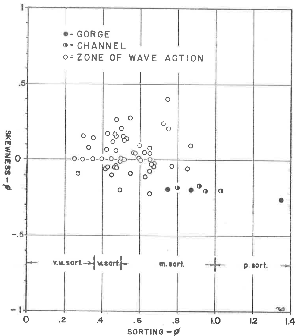
Figure 6. Comparison of sorting and skewness.
