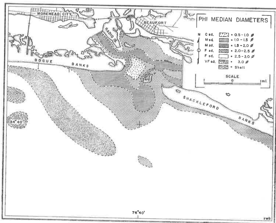
Figure 4. Distribution of phi median diameters
