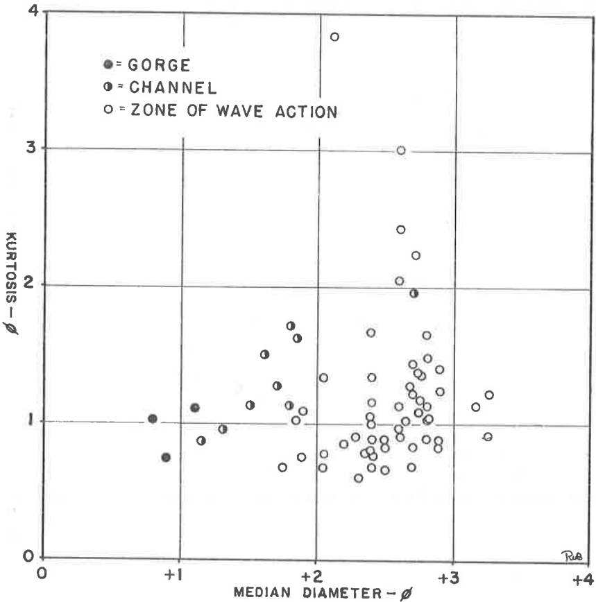
Figure 8. Comparison of kurtosis and median diameters
