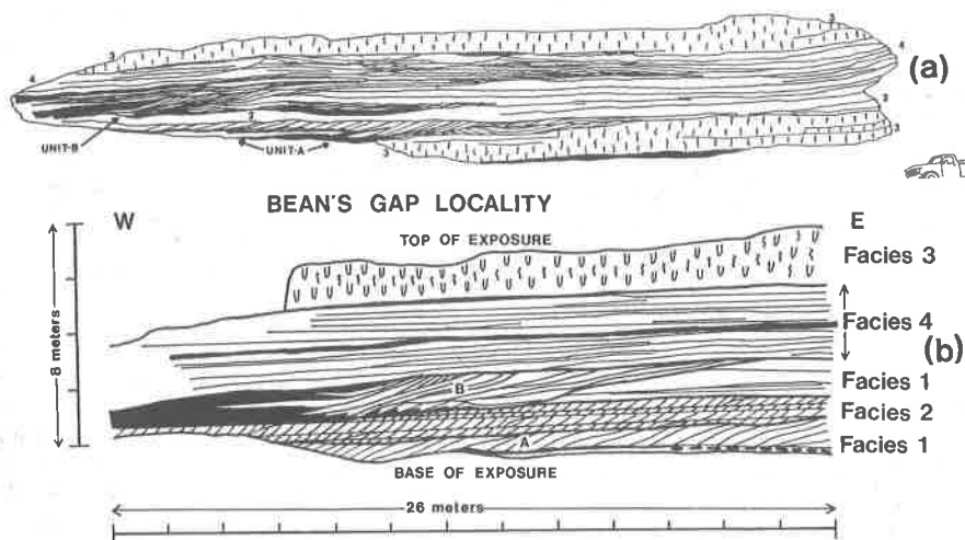
Figure 6 (a). Outcrop sketch showing lateral and vertical relationships between the four Clinch Sandstone facies defined and described in text. Note locations of two laterally persistent Facies 1 trough cross-set units, labelled A and B, which are discussed in detail in this study. Length of outcrop is 75 m, height is 10 m. (b) Detailed sketch of western half of outcrop depicted in sketch in Figure 6a, showing lateral and vertical relationships between the four Clinch Sandstone facies. Facies units are defined and described in text. Note two laterally persistent Facies 1 trough cross-set units, labelled A and B, which are discussed in detail in this study and are shown in Figure 7.
