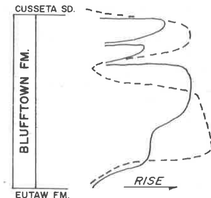
Figure 7. Relative sea-level curves for the age-equivalent Blufftown Formation of east Alabama. Dashed curves from Reinhardt (1980); solid is from Skotnicki (1985). The three cycles of Skotnicki likely correspond to the changes shown in Figure 6.
