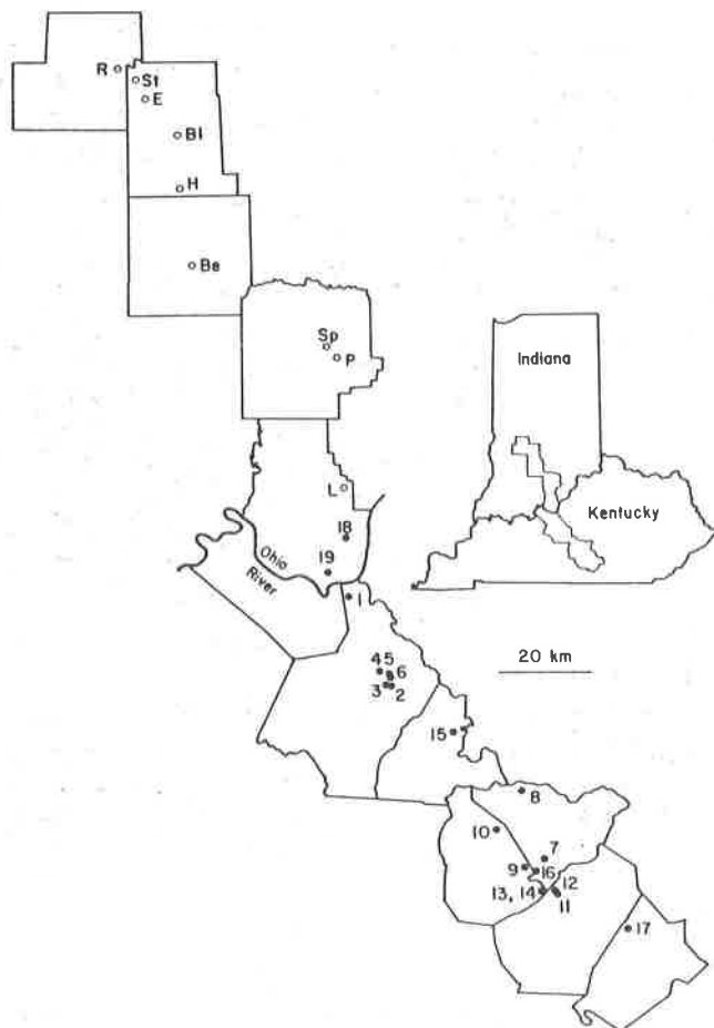
Figure 2. Map of localities used in this study. Open circles represent the limestone localities collected by Cumings and others (1906) and closed circles represent shale localities collected for this study. R, Ramona; St, Stinesville; E, Ellettsville; Bl, Bloomington; H, Harrodsburg; Be, Bedford; Sp, Spergen Hill; P, Paynter's Hill; L, Lanesville.
