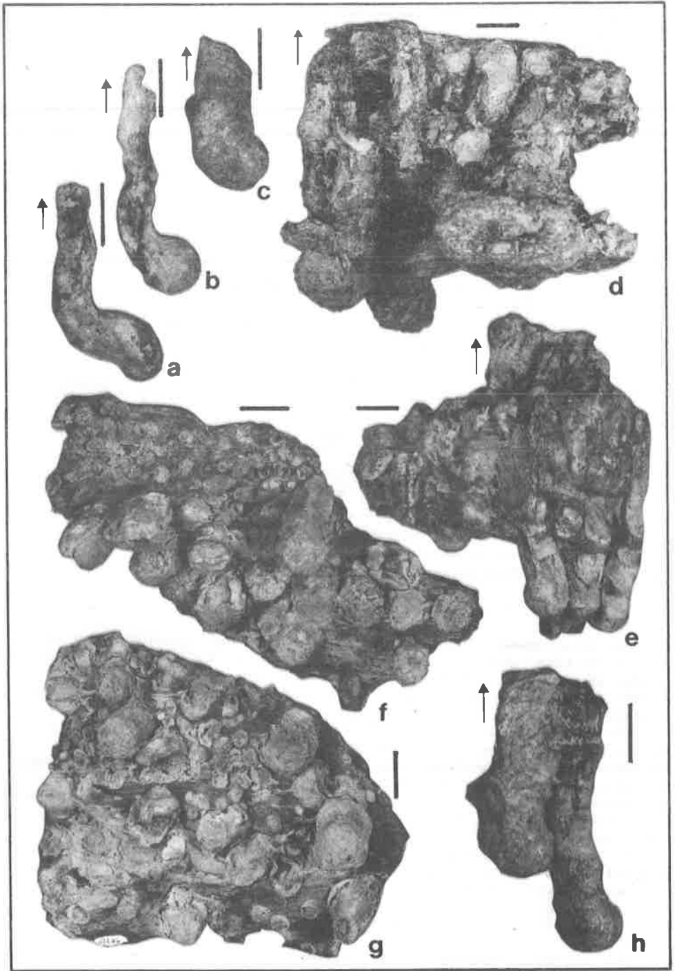
Figure 4. (a,b) Distorted Teredolites tubes in side view. (c) Distal end of Teredolites tube. (d,e,h) Teredolites clusters in side view. (f,g) Teredolites clusters in basal plan view. Note: Scale Bar = 2 cm., arrows indicate "up".
