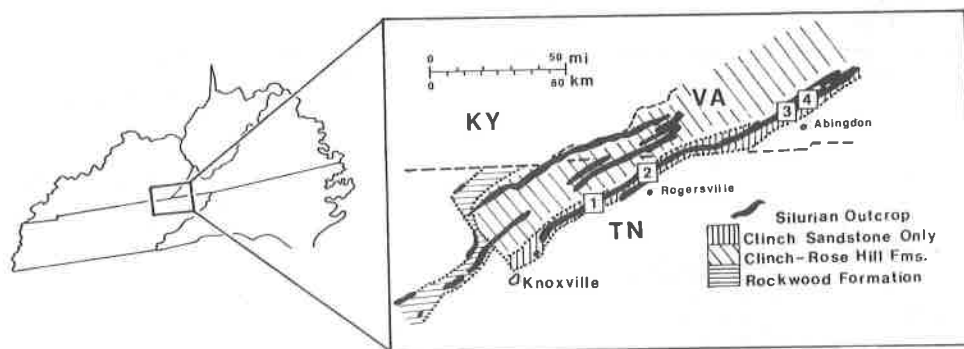
Figure 4. Location of Silurian outcrop belts in the Valley and Ridge Province of northeastern Tennessee and southwestern Virginia. Locality 1 (Beans Gap) is the focus of this study. Modified from Miller (1976).
