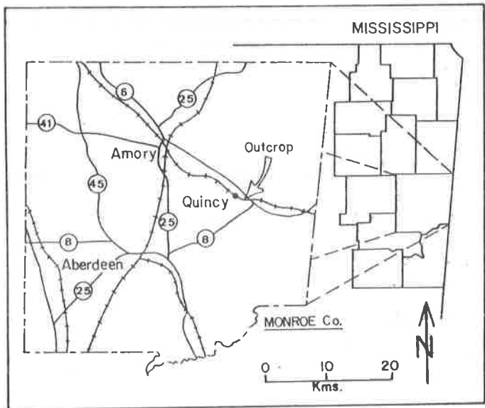
Figure 1. Location Map of Teredolites Outcrop.
