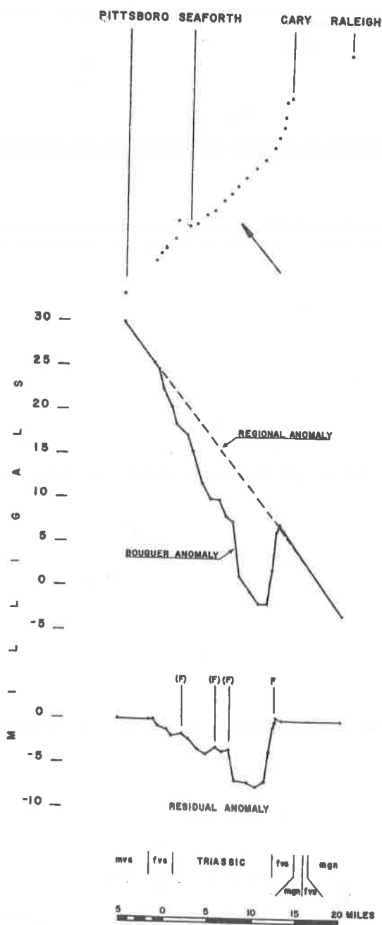
Figure 7. Gravity profile along traverse from Pittsboro through Cary to Raleigh
