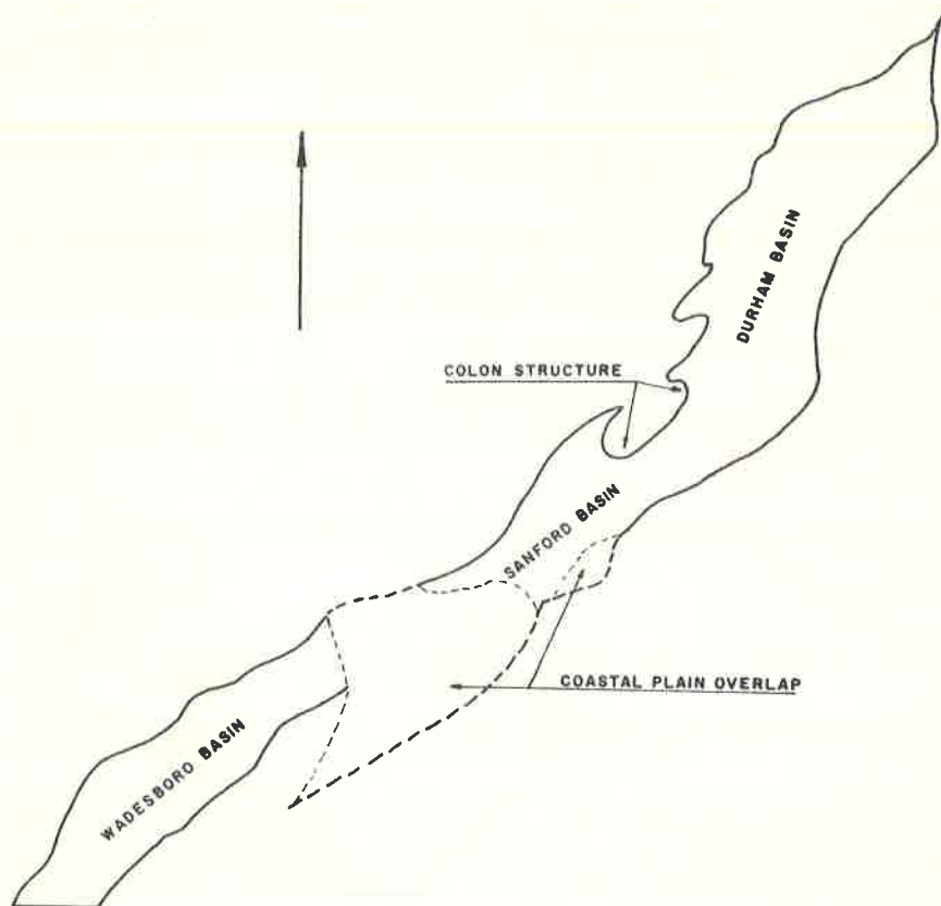
Figure 2. Sketch Map of the Deep River-Wadesboro Triassic basin showing the location of the four structure units: Durham basin, Color Cross Structure, Sanford basin, and the Wadesboro basin.
