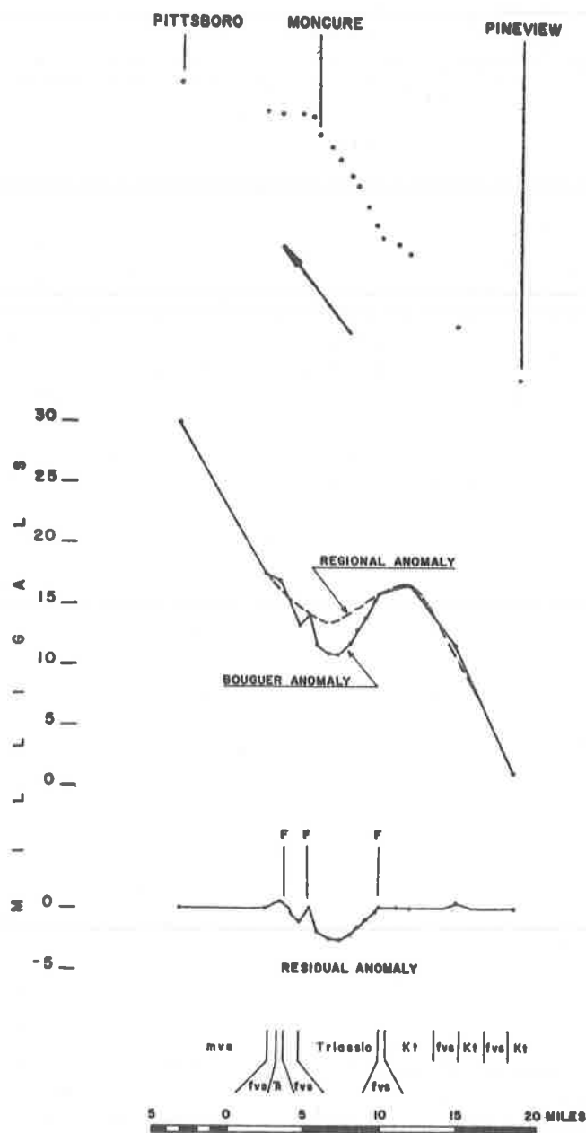
Figure 8. Gravity profile along traverse from Pittsboro through Moncure to Pineview.
