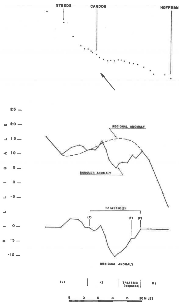
Figure 11. Gravity profile along traverse from Steeds through Candor to Hoffman.
