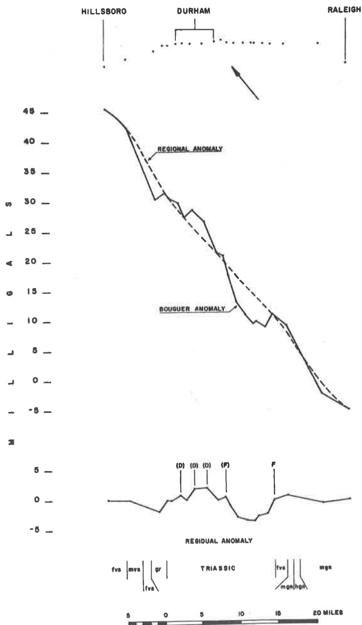
Figure 6. Gravity profile along traverse from Hillsboro through Durham to Raleigh
