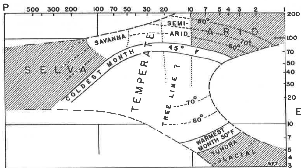
Figure 3. A climatic generalization of the station data shown in Figs. 1 and 2, with approximate boundaries indicated for: warm climate (coldest month 45^{\circ}\text{F} ), cold climate (warmest month 50^{\circ}\text{F} ), and the tree line. The class labels represent a geomorphic interpretation. It is not felt, however, that rigorous conclusions can be drawn from the data; boundaries shown are not precise, but are included for information because of the wide use of boundaries of this type in the past.
