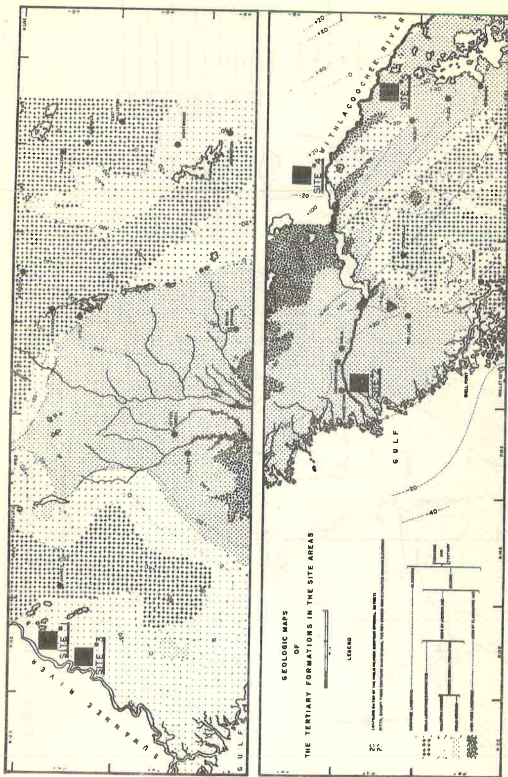
Figure 12. Five sites in the Citrus-Levy County area.
