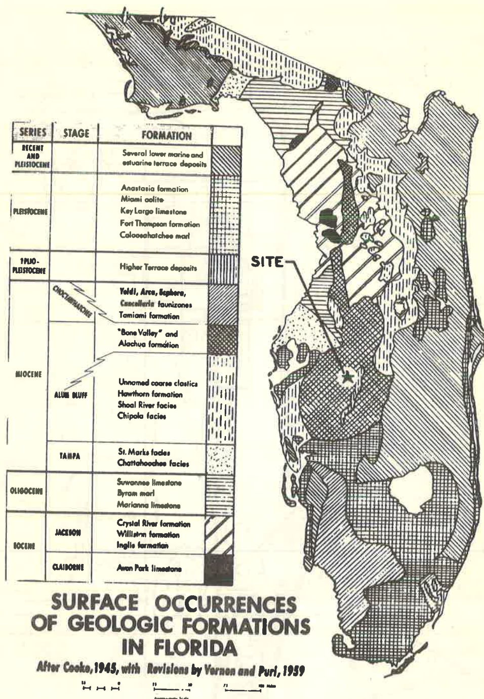
Figure 4. Geologic map of Florida indicating surface occurrences at nuclear reactor site.
