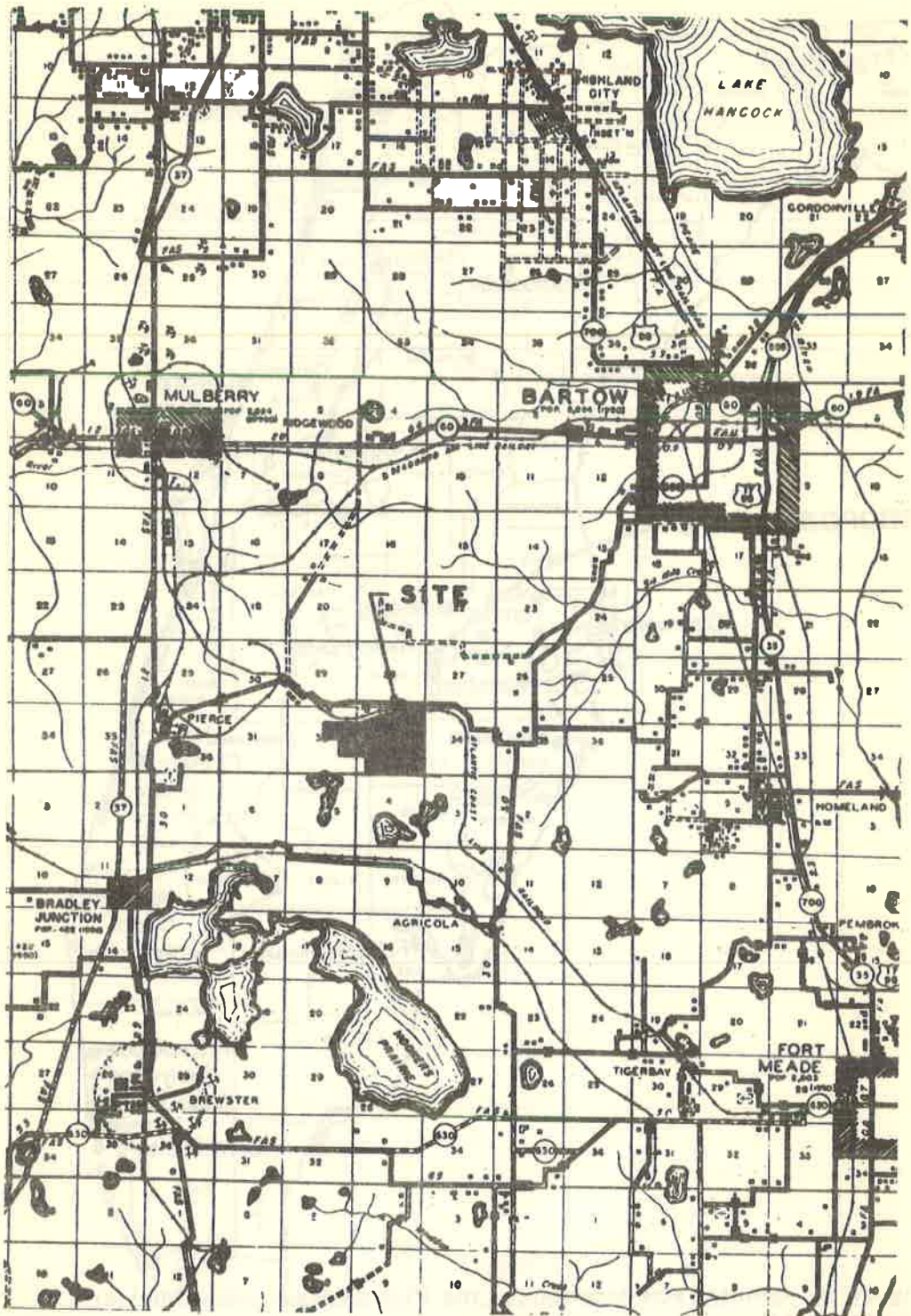
Figure 2. Area immediately surrounding the nuclear reactor site.
