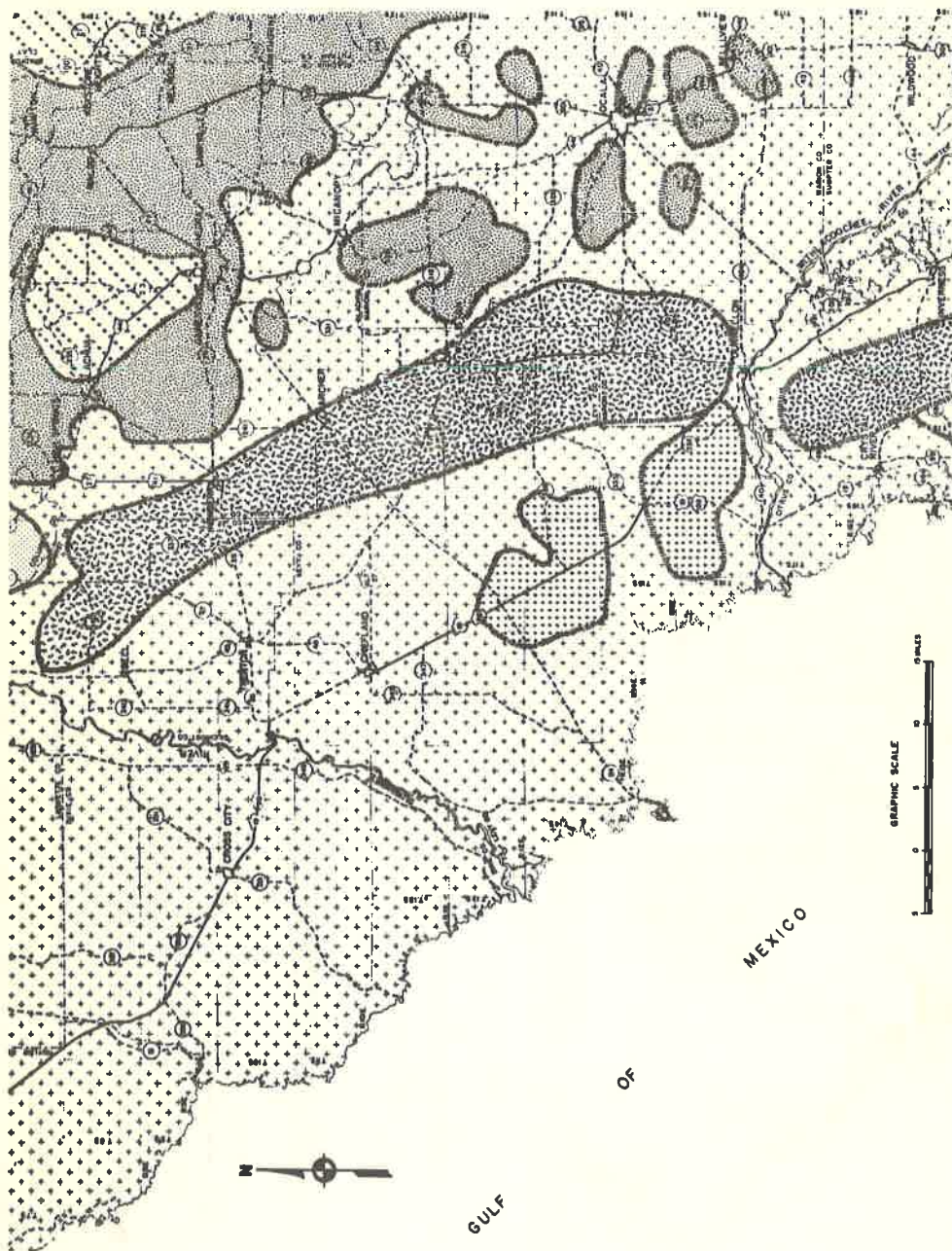
Figure 11. Detailed geology of the Citrus and Levy Counties, (Vernon, 1951).
